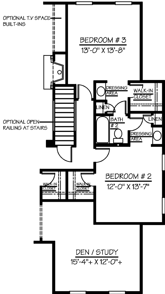
PARTIAL FIRST FLOOR PLAN OPTIONAL DEN / STUDY PLAN
